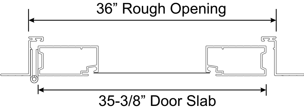
Single Zeus Door
