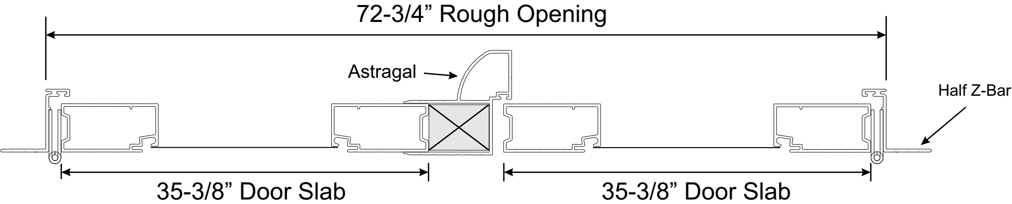
Two ZEUS ® Doors French Door Configuration
